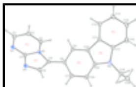
Fig. 1. A molecular structure of (I) with 30% probability displacement ellipsoids, showing the atom-numbering scheme employed.
